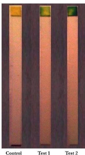
Fig. 5 Glucose water phantom from mp3 – Modulated Broadband Electromagnetic Radiation
